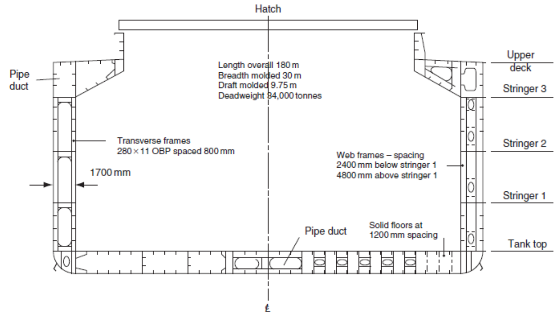
Fig. 17.8 Bulk carrier—double-side skin midship section.
