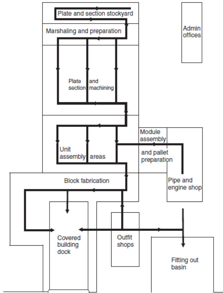
Figure 11.4 Shipyard layout.
