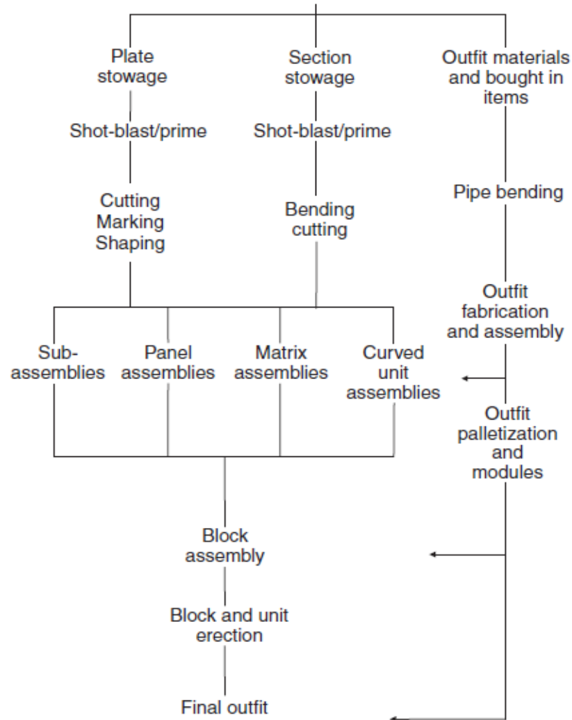
Figure 11.3 Shipbuilding process.
