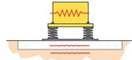
Machine on isolators on the floor, no foundation
